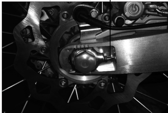
Tendeur regulation
